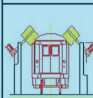
ROOF BRUSHES MODEL FIRAT LINE 435 RB FIRAT LINE 535 RB FIRAT LINE 441 RB FIRAT LINE 541 RB
