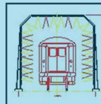
RINSING ARCH MODEL FIRAT LINE 435 RA FIRAT LINE 535 RA FIRAT LINE 441 RA FIRAT LINE 541 RA
